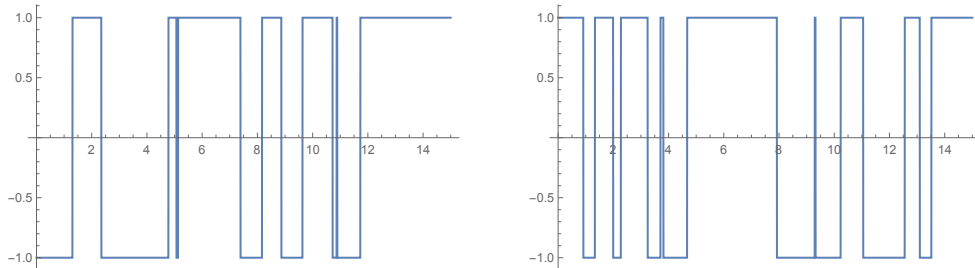
Figure 8: Sample realizations of the switching process from Example 1.8 with the symmetric alternative distribution of the random variable A .
