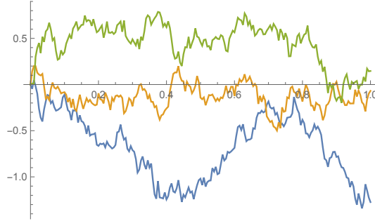
Figure 6: Sample realizations of the Ornstein-Uhlenbeck process, see Example 1.6.
